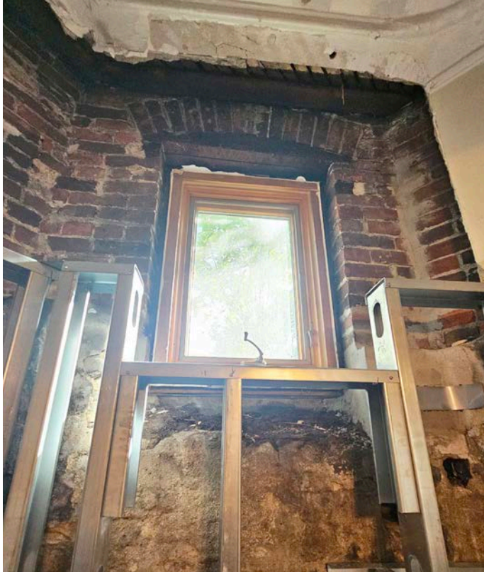
Basement West Wing - Before Renovation
